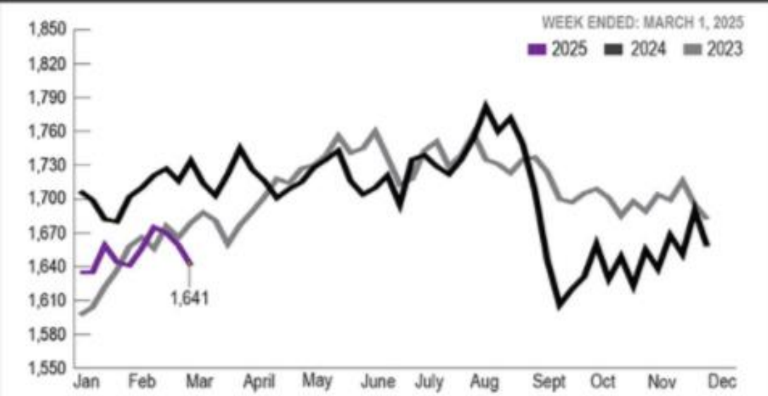
WEEKLY TONNAGE OF CRUDE STEEL PRODUCTION (thousands of net tons)
